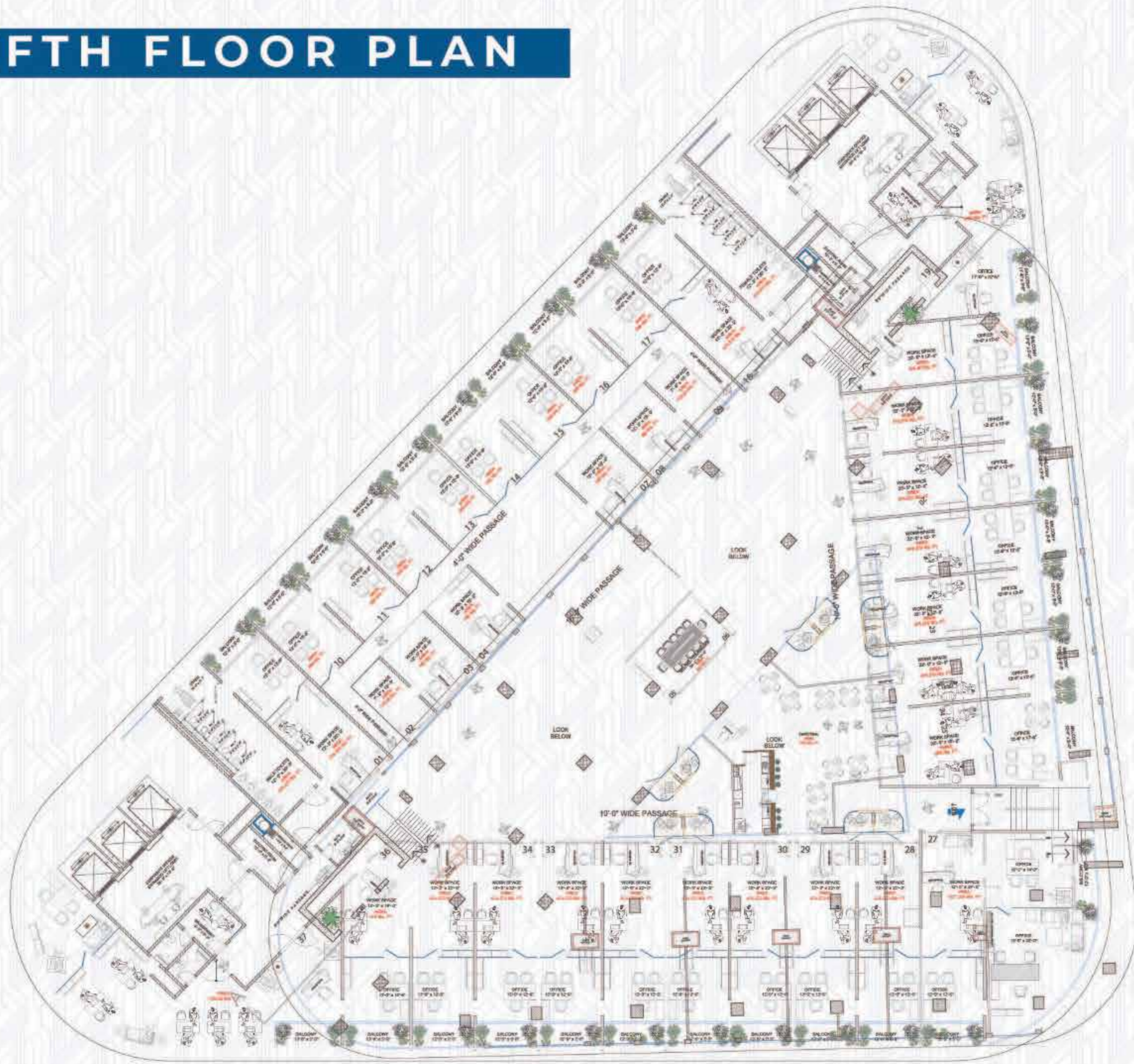
5TH FLOOR PLAN OFFICE BLOCKS
