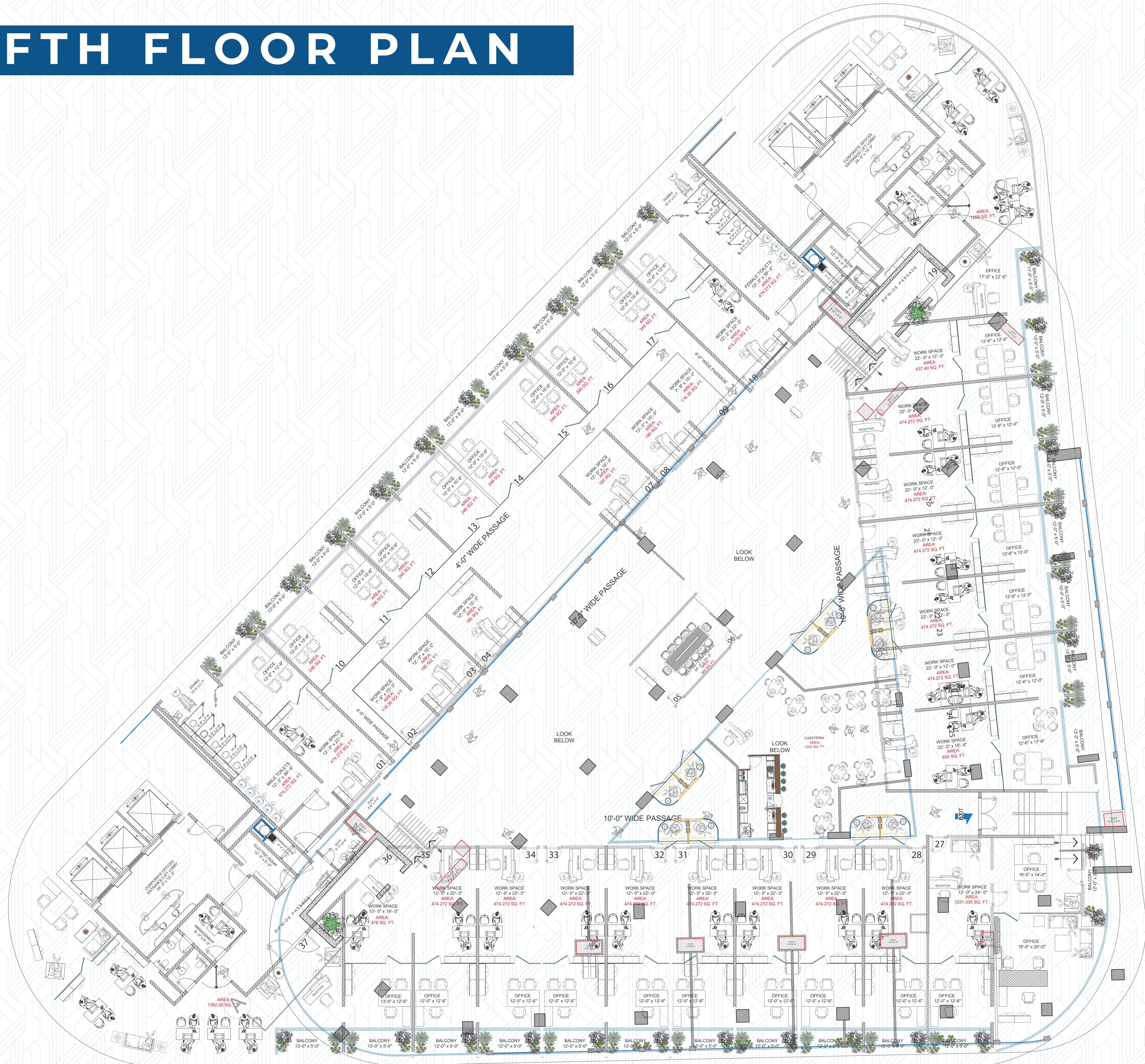
5TH FLOOR PLAN OFFICE BLOCKS
