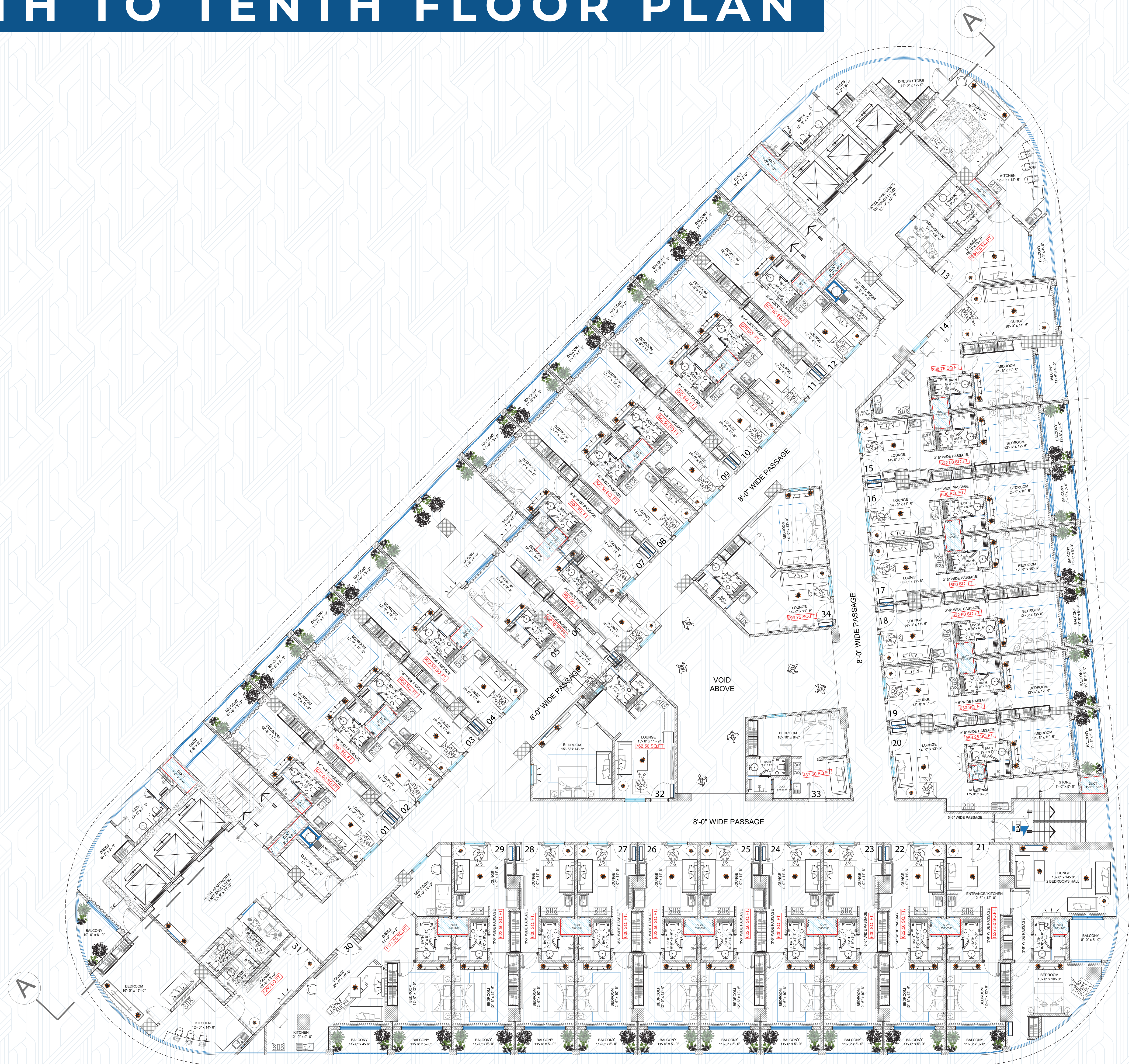
6TH TO 10TH FLOOR PLAN APARTMENT BLOCKS
